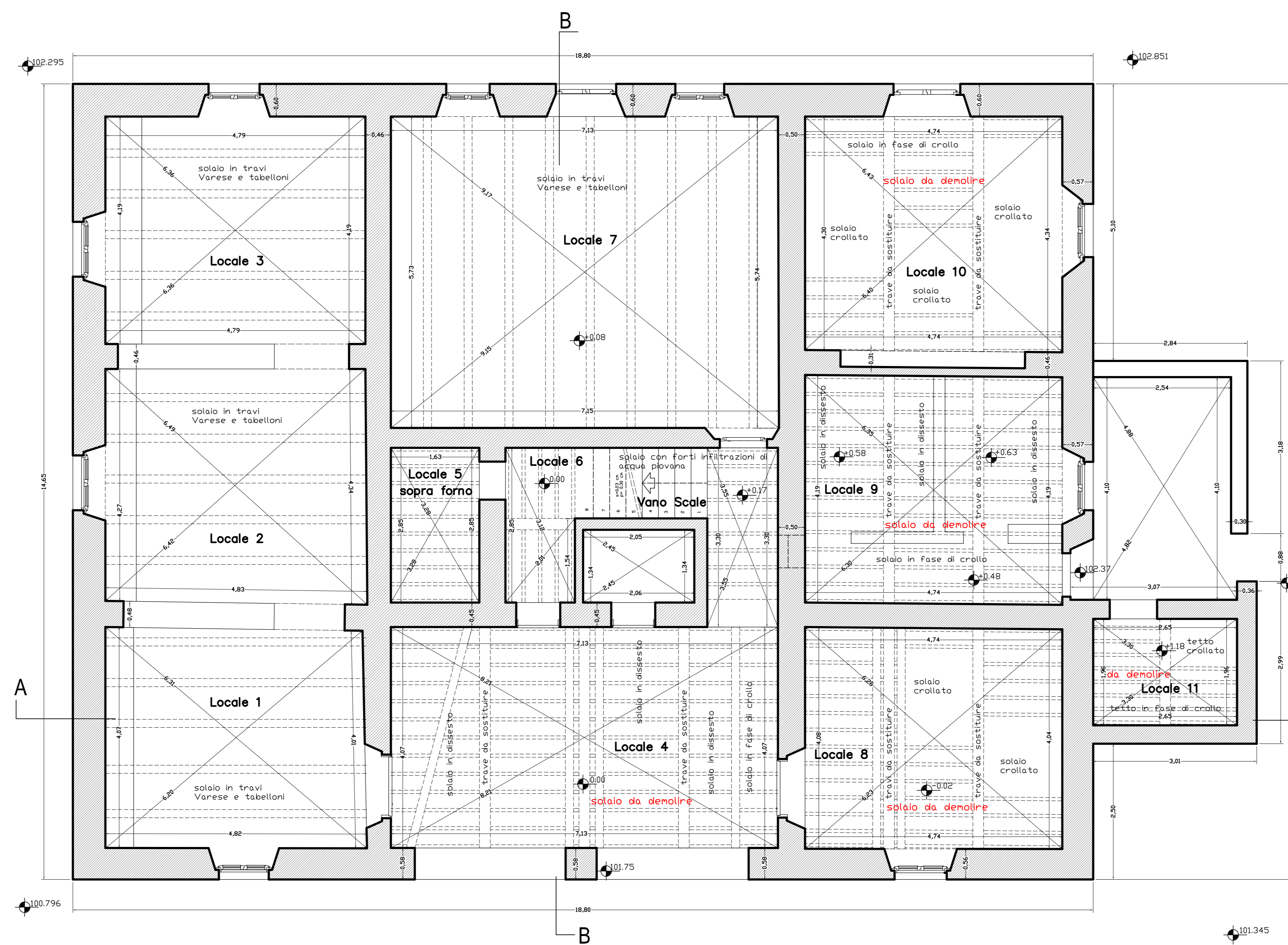
PIANO TERRA
